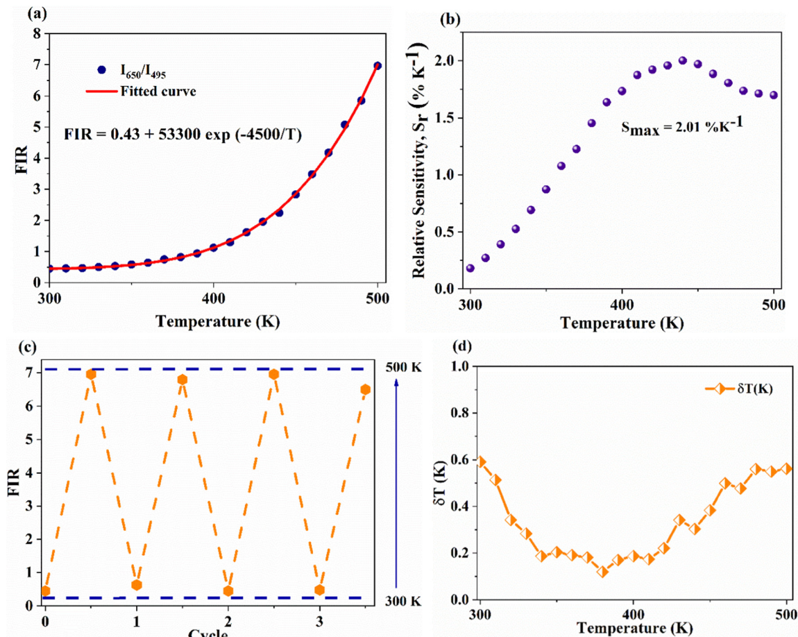
Fig. 7 (a) and (b) Variation of \text{FIR} \frac{I_{650}}{I_{495}} and relative sensitivity, S_r , with temperature, (c) temperature cycling of FIR, and (d) the temperature resolution in the temperature range 300–500 K.
