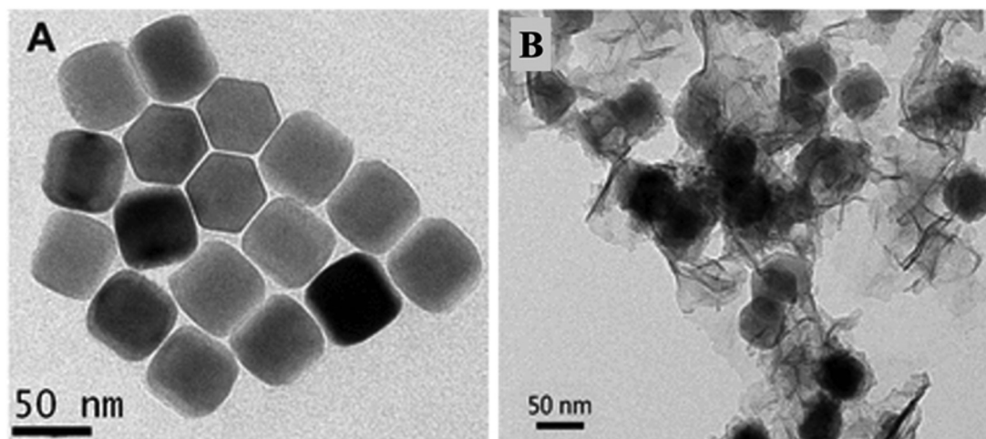
Fig. 13 TEM images (A) of OA-capped \text{NaYF}_4:\text{Yb,Tm}@NaYF_4 core shell UCNPs, and (B) of \text{MnO}_2 NS-modified \text{NaYF}_4:\text{Yb,Tm}@NaYF_4 UCNP assemblies. 67 Copyright©2015, American Chemical Society.
