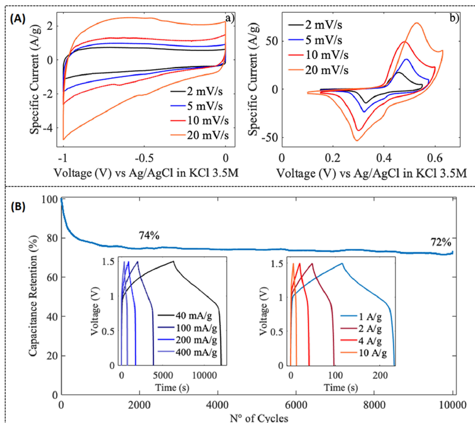
Fig. 16 (A) (a and b) CV response of TGO and Ni-TGO at different scan rates, (B) capacitance retention response of ASCs over 10 000 cycles at 1 \text{ A g}^{-1} current density inset: with GCD curves at different applied current density. Reprinted with permission, 97 Copyright (2022) from Elsevier.
