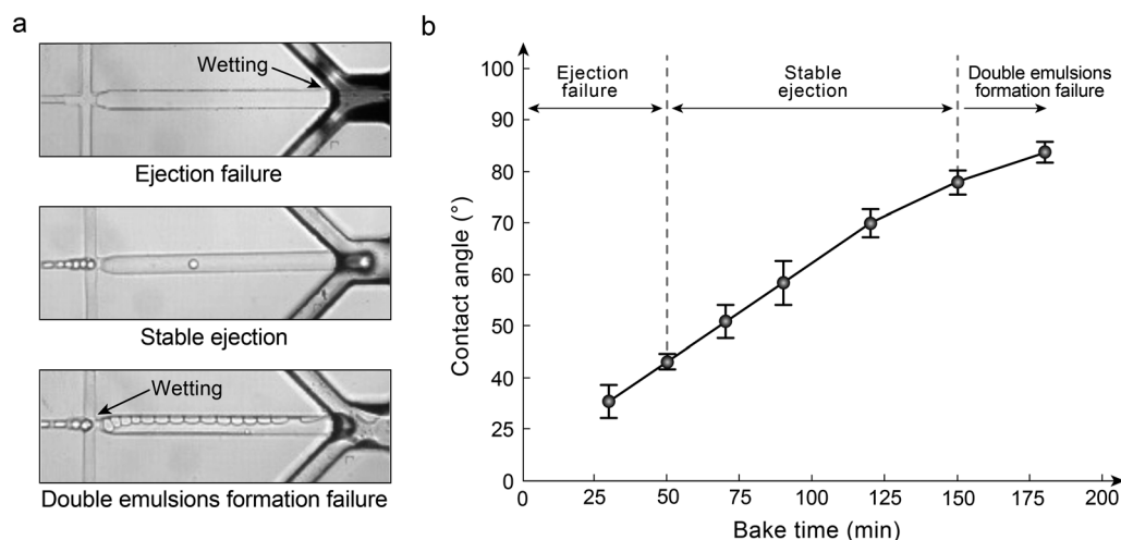
Fig. 2 Spatial wettability patterns enable stable generation and ejection of double emulsions. (a) Images showing three conditions of double emulsion formation and ejection in the microfluidic device with different wettability patterns. (b) The corresponding intrinsic contact angle in the microfluidic channel for the three ejection conditions shown in (a). Stable generation and ejection of double emulsions occur within a contact angle range of \sim 35^\circ to 83^\circ .
