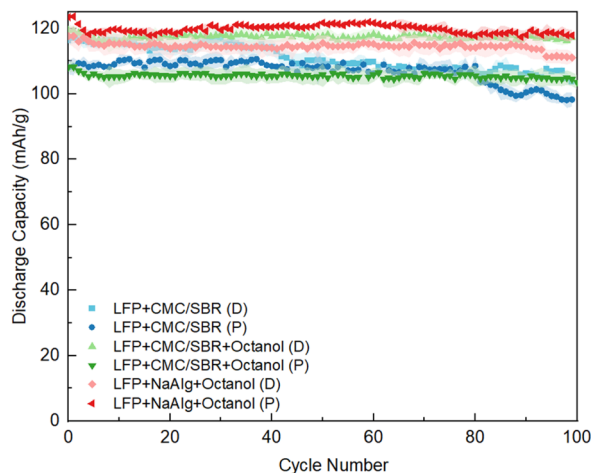
Fig. 5 The cycling performances of the samples involved in this project tested after 100 cycles. Here D is short for draw-down electrodes, P is short for printed electrodes; the shades of each plot indicate the error bars.
