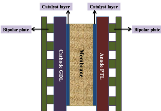
Fig. 9 Core components of a PEM electrolyser cell; PTL = porous transport layer; GDL = gas diffusion layer. Modified from ref. 185 with permission from IOP Publishing, copyright 2021.
