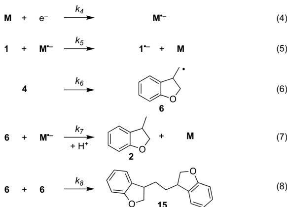
Scheme 6 Reaction steps in the mediated electroreductive cyclisation of aryl iodide 1 , including dimerisation of alkyl radical 6 .
