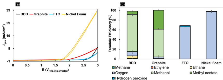
Fig. 1 Effect of different electrodes on (non-)Kolbe electrolysis: (a) CV of BDD, graphite, FTO and nickel foam conducted in 1 M acetic acid/sodium acetate at pH 5; (b) average FE towards (non-)Kolbe/Hofer–Moest/indirect oxidation products during electrolysis of 1 M acetic acid/sodium acetate for 50 minutes in a batch cell at 25 mA cm -2 and pH 5.
