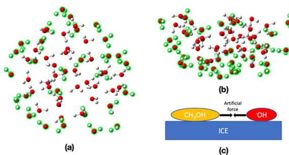
Fig. 2 (a) Top and (b) side views of the ice cluster model employed in this study. The water molecules highlighted in green were frozen during the structure optimization. (c) Adding artificial force between the \text{CH}_3\text{OH} and OH radical on ASW.
