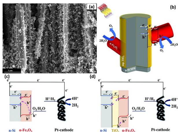
Fig. 24 SEM image (a) and schematic diagram (b) of the n-Si nanowires/ \text{TiO}_2 / \alpha\text{-Fe}_2\text{O}_3 . Band alignment of n-Si/ \alpha\text{-Fe}_2\text{O}_3 (c) and n-Si/ \text{TiO}_2 / \alpha\text{-Fe}_2\text{O}_3 (d). Reproduced with permission from ref. 155, Copyright © The Royal Society of Chemistry 2020.
