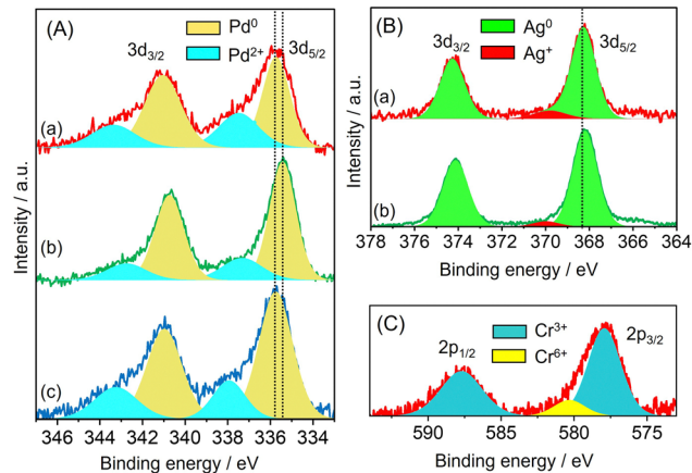
Fig. 2 (A) Pd 3d XPS spectra of (a) PdAgCr/amine-MS-C, (b) PdAg/amine-MS-C and (c) Pd/amine-MS-C; (B) Ag 3d XPS spectra of (a) PdAgCr/amine-MS-C and (b) PdAg/amine-MS-C; and (C) Cr 2p XPS spectrum of PdAgCr/amine-MS-C.
