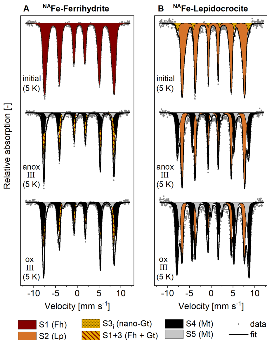
Fig. 3 Mössbauer spectra collected at 5 K from (A) NA Fe-ferrihydrate and (B) NA Fe-lepidocrocite mesh bags without soil before the incubation (initial) and after the incubation in the redox fluctuating mesocosms (redox cycle III anoxic and oxic period). Averaged fitting parameters and interpretations of Mössbauer fit components are given in Table 1, all fitting parameters are presented in Tables S11 and S12.† Abbreviations: anox = anoxic, ox = oxic, S = sextet.
