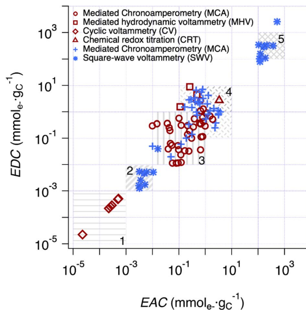
Fig. 5 Comparison of EDC and EAC values of chars and pyDOM samples between this study and prior work. The red enclosed symbols ( i.e. \square , \diamond , \triangle and \circ ) are the values derived from chars in previous studies, 37,41,49,50,86–90 while the blue unenclosed symbols ( i.e. \times , + and * ) are the values derived from pyDOM samples in previous studies 24,25,27 and this study. Regions 2 and 5 are the SWV results from the same samples using faradaic and calibrated quantifications, respectively. Five regions were highlighted ( i.e. , Region 1 to 5) for categorization of the values.
