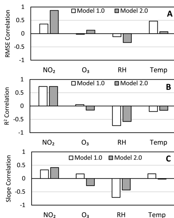
Fig. 7 (A) RMSE, (B) R 2 , and (C) slope correlations for the Model 1.0 and Model 2.0 calibrations to FRM NO 2 , FEM O 3 , internal sensor relative humidity, and internal sensor temperature.
