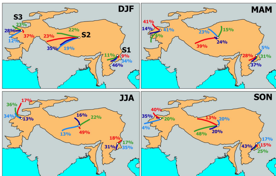
Fig. 3 Three-day backward air-mass trajectory clusters at three receptor sites S_1 ( 27^\circ \text{N} , 102^\circ \text{E} ), S_2 ( 33.5^\circ \text{N} , 88^\circ \text{E} ) and S_3 ( 36.2^\circ \text{N} , 67^\circ \text{E} ) for the year 2018 in the TP. The seasons are defined as winter (December–January–February, DJF), spring (March–April–May, MAM), summer (June–July–August, JJA) and autumn (September–October–November, SON).
