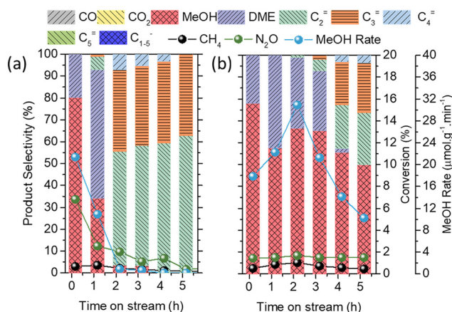
Fig. 6 Stability test of the (a) 5Cu/AEI-C and (b) 5Cu/AEI-S zeolite catalysts in the cDMTM reaction at 350 °C. Reaction conditions: 100 mg catalyst, CH 4 /N 2 O/H 2 O/Ar = 10/10/2/28 ml min -1 , SV = 30 000 ml g -1 h -1 .
