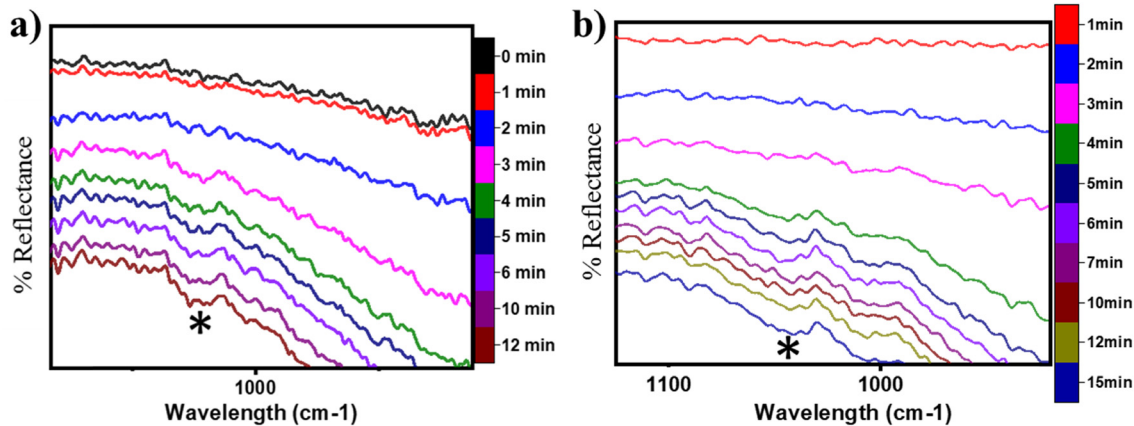
Fig. 16 DRIFT spectra at successive time intervals for the HC–O stretching region for (a) CH 4 oxidation on moist CuO at 300 °C and b) CH 4 oxidation on dry CuO at 300 °C. Symbols: (*) 1050 cm -1 .
