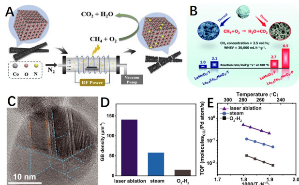
Fig. 12 (A) Schematic diagram of N_2 plasma-treated Co_3O_4 catalyst. Reproduced from ref. 140 with permission from Elsevier. (B) Diagram of O_2 atmosphere glow discharge plasma-treated LaMnO_3 and Ce-LaMnO_3 catalyst. Reproduced from ref. 199 with permission from the Royal Society of Chemistry. (C) High-resolution TEM image of laser ablation-generated Pd NPs. The orange dashed lines highlight \Sigma 3(111) TBs, and the blue dash lines highlight GBs; (D) GB density statistical histogram of laser-generated Pd/Al_2O_3 and Pd/Al_2O_3 after steam (600 °C) and O_2-H_2 pretreatments; (E) Arrhenius plots of methane combustion of laser-generated Pd/Al_2O_3 and Pd/Al_2O_3 after steam (600 °C) and O_2-H_2 pretreatments. TOF, turnover frequency. Reproduced from ref. 77 with permission from the American Association for the Advancement of Science.
