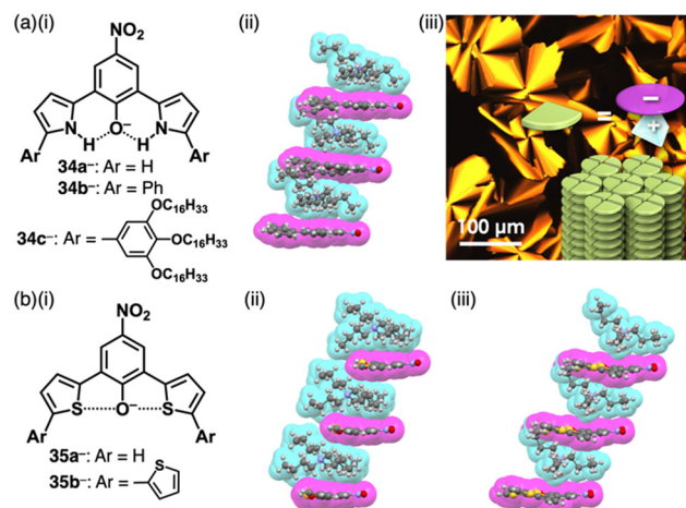
Fig. 21 (a) (i) Deprotonated dipyrrolynitrophenols 34\text{a-c}^- , (ii) single-crystal X-ray structure of \text{TBA}^+ \cdot 34\text{b}^- and (iii) POM image of \text{TBA}^+ \cdot 34\text{c}^- at 65^\circ\text{C} upon cooling (redrawn from ref. 67b. Copyright 2018 Wiley) and (b) (i) deprotonated dithienynitrophenols 35\text{a,b}^- and single-crystal X-ray structures of (ii) \text{TBA}^+ \cdot 35\text{a}^- and (iii) \text{TBA}^+ \cdot 35\text{b}^- . The crystal structures are redrawn from cif files: 1830529, 2253150 and 2253154.
