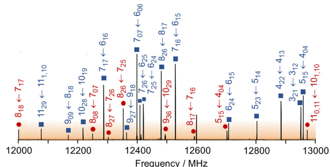
Fig. 2 Broadband scan in the frequency region from 12 to 13 GHz. The C_1 conformer is labeled with blue squares and the C_s conformer with orange circles. Each caption gives the quantum numbers J , K_a , K_c . The intensities are in arbitrary units.
