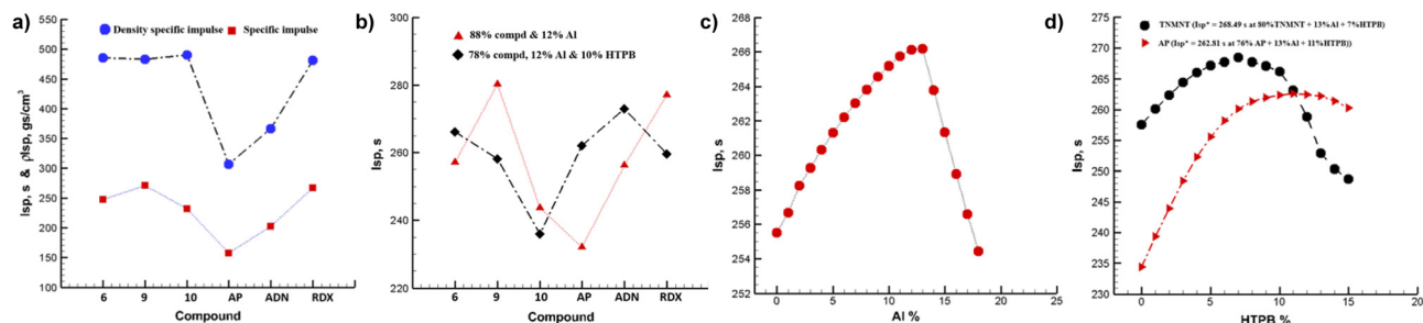
Fig. 3 (a) Comparison of propulsive properties (a) monopropellant (b) composite bipropellant. (c) TMNT at 10% HTPB and varying the percentage of TMNT (90–72%) and Al (0–18%). (d) TMNT and AP at 13% Al and varying the percentage of TMNT/AP (87–71%) and HTPB (0–16%).
