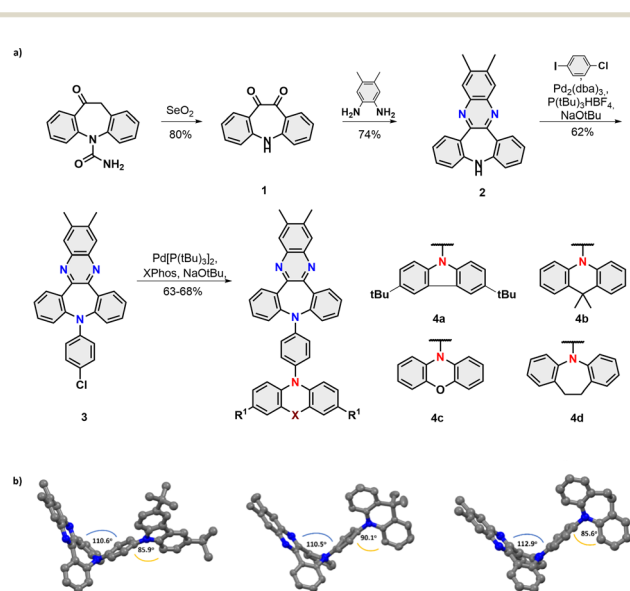
Fig. 2 (a) Synthetic route towards title compounds 4a–d ; (b) Single X-ray structure of the dyes 4a,b , and d .
