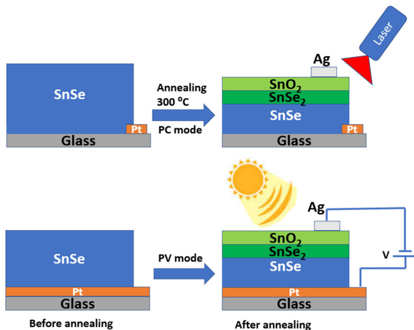
Fig. 1 Upper and lower sections: device structures implemented by open-air annealing for PC and PV, respectively, of SnSe at 300 °C for a defined time.
