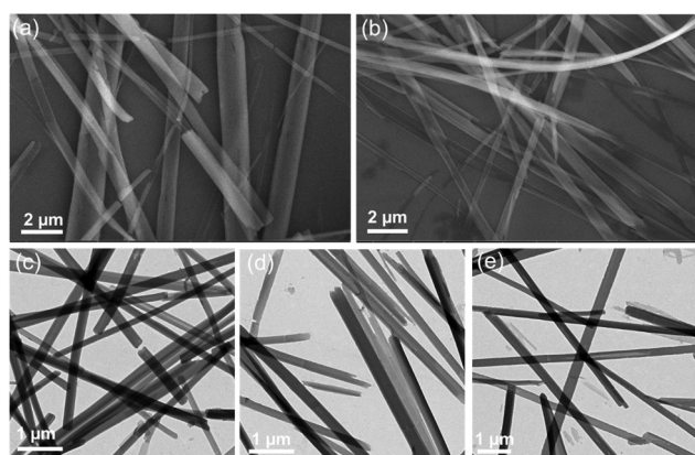
Fig. 5 SEM images of nanostructures formed in DMSO solutions of (a) \text{Cs}^+[\text{Eu}(+)-\text{tfac}]_4^- and (b) \text{Na}^+[\text{Eu}(+)-\text{tfac}]_4^- . TEM images of the self-assembled aggregates formed from (c) \text{Cs}^+[\text{Eu}(+)-\text{tfac}]_4^- , (d) \text{Rb}^+[\text{Eu}(+)-\text{tfac}]_4^- and (e) \text{K}^+[\text{Eu}(+)-\text{tfac}]_4^- .
