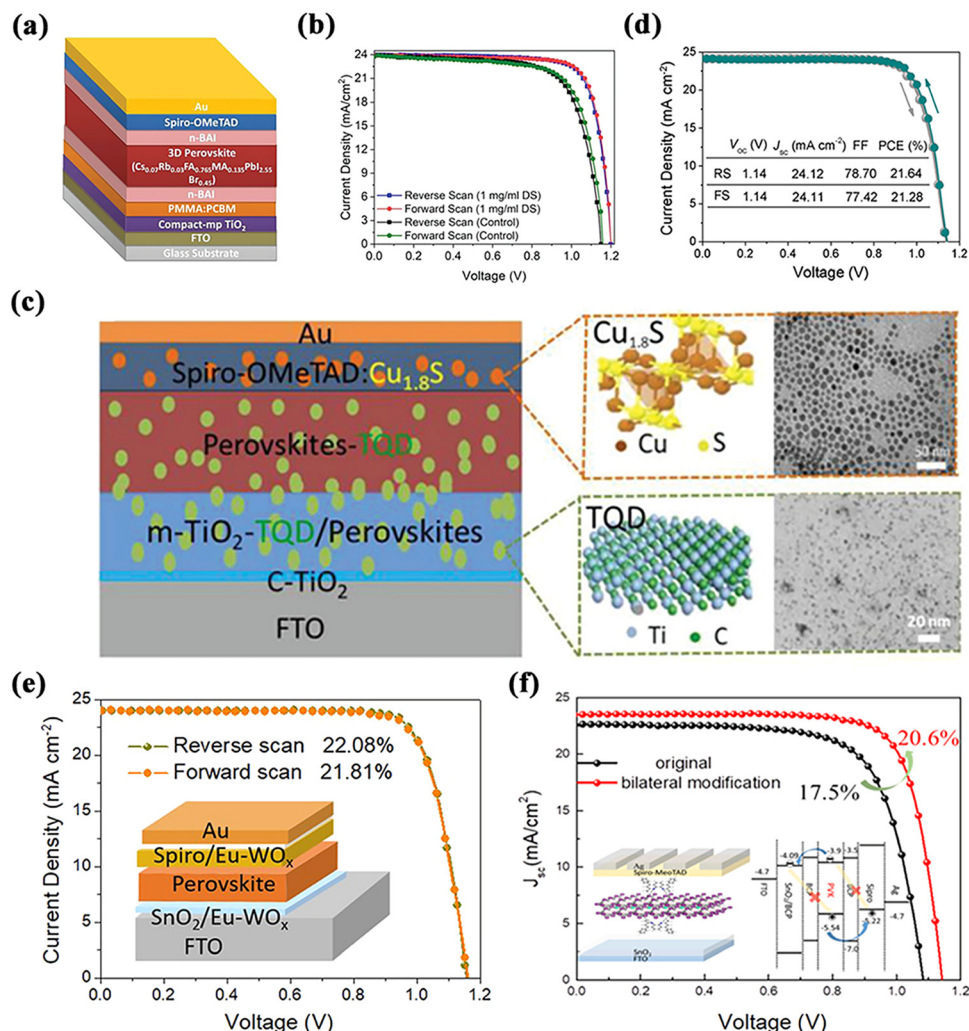
Fig. 15 Schematic diagram of the structure of dual-interface-modified PSCs (a) and J-V curves (b) based on n-BAI. Reproduced with permission from ref. 141. Copyright 2019 Wiley. Modification with TQD and Cu_{1.8}S (c) and J-V curves (d) based on this device architecture. Reproduced with permission from ref. 142. Copyright 2020 Wiley. (e) Structure and J-V curves of dual-interface-modified PSC with Eu-WO_x . Reproduced with permission from ref. 143. Copyright 2021 Elsevier. (f) Structure and J-V curves of dual-interface-modified PSC with BCP. Reproduced with permission from ref. 144. Copyright 2021 American Chemical Society.
