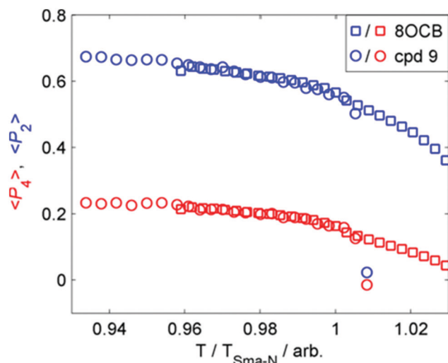
Fig. 4 Plot of the first two even ( P_n ) order parameters as a function of reduced temperature ( T/T_{\text{SmA-N}} ) for compound 9 (circles) and 8OCB (squares).
