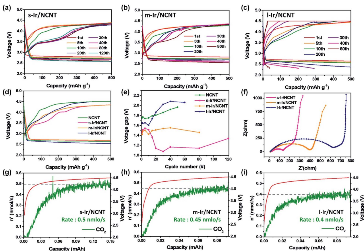
Fig. 5 Electrochemical cell data of NCNTs and s-, m- and l-Ir/NCNTs: (a–c) cycling performance of Li–CO 2 cells fabricated using s-, m-, and l-Ir/NCNTs loaded electrodes measured at 50 mA g carbon −1 with a limited capacity of 500 mA h g carbon −1 . (d) Discharge/charge curves during the 15th cycle. (e) Voltage gap graphs calculated during the discharge and charge reactions for Li–CO 2 cells at 250 mA h g −1 during each cycle. (f) EIS profiles of the s-, m- and l-Ir/NCNT-containing electrode after 10 cycles. (g–i) in situ DEMS results of the gas evolution rate for CO 2 during charging in cells with s-, m- and l-Ir/NCNTs.
