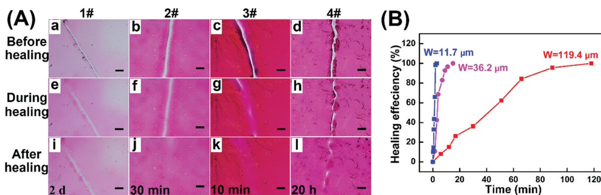
Fig. 5 (A) Microscope images of self-healing in ambient environments for hydrogel coatings with the corresponding experiment parameters in Table 1 (Scratch width: about 25 \mu\text{m} , scale bar: 100 \mu\text{m} ). (B) Healing curves of hydrogel coatings (3# sample in Table 1) with different scratch widths of 11.7, 36.2 and 119.4 \mu\text{m} .
