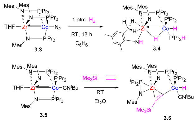
Scheme 15 The reactivity of a tris(phosphinoamido) Zr/Co complex in H 2 and terminal alkyne activation.
