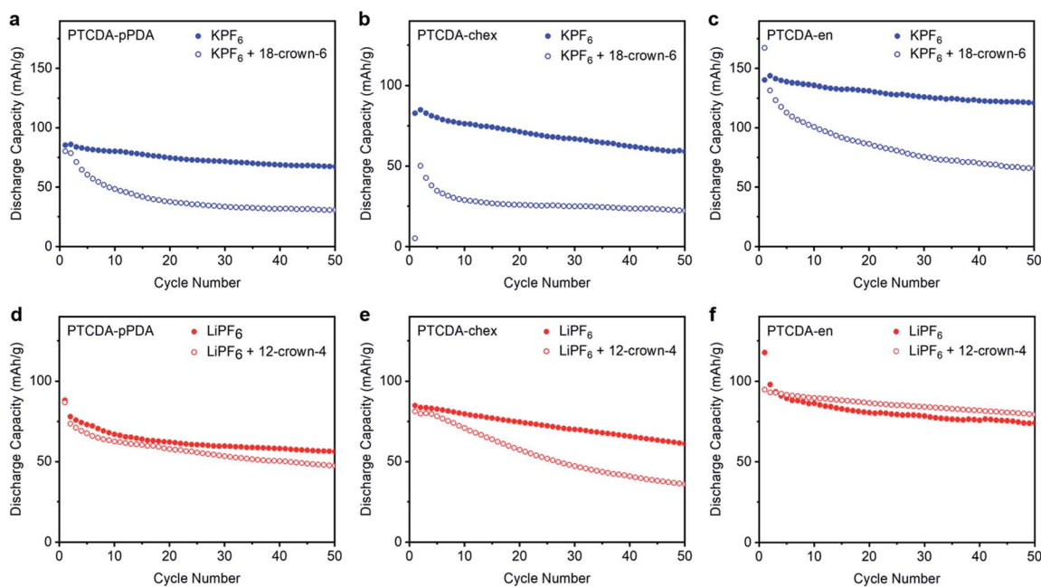
Fig. 5 Cycling performance at 100 \text{ mA g}^{-1} for (a) PTCDA-pPDA , (b) PTCDA-chex , and (c) PTCDA-en in metal half cells containing 0.8 \text{ M KPF}_6 with and without 0.8 \text{ M 18-crown-6} ether and (d) PTCDA-pPDA , (e) PTCDA-chex , and (f) PTCDA-en in cells containing 1.0 \text{ M LiPF}_6 with and without 1.0 \text{ M 12-crown-4} ether.
