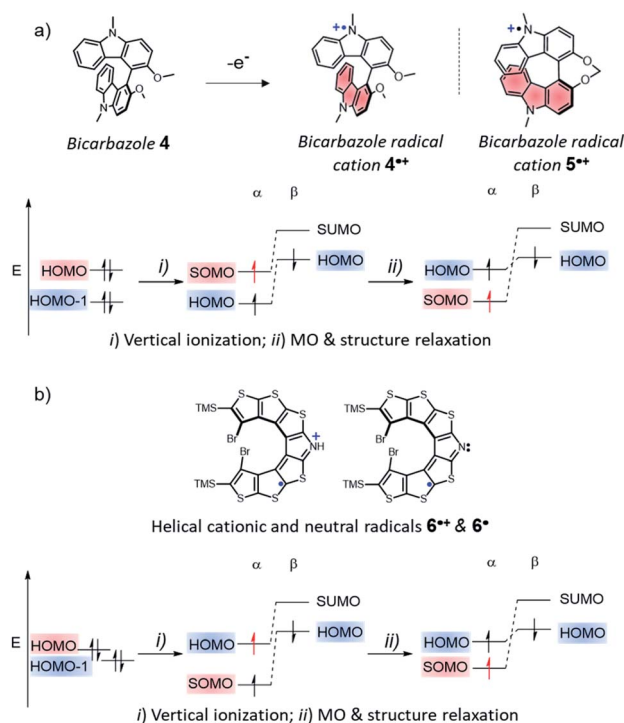
Fig. 5 Chemical structures of (a), the bicarbazole radical cations 4^{+\cdot} and 5^{+\cdot} and (b), the cationic radical aza-thia[7]helicene 6^{+\cdot} and neutral aza-thia[7]helicene 6^{\cdot} , with a schematic illustration of the steps leading to SHI.
