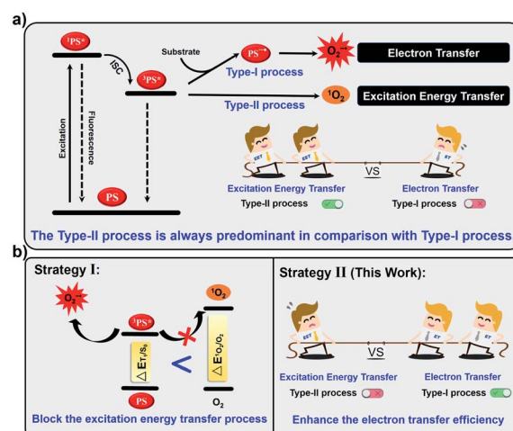
Fig. 1 (a) The competition between excitation energy transfer and electron transfer in PDT. (b) The strategies for the design of type-I PSs: reported strategy (left) and proposed strategy in this work (right).
