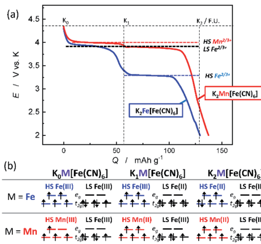
Fig. 14 (a) Typical discharge curves of KFeFe–PBA and KMnFe–PBA in K cells. (b) Electronic structures of K_xM[Fe(CN)_6]_x , where x = 0, 1, 2 , and M = Fe or Mn .
