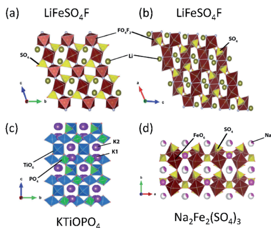
Fig. 11 Typical compounds representing (a) tavorite, (b) triplite, (c) \text{KTiOPO}_4 , and (d) alluaudite types.
