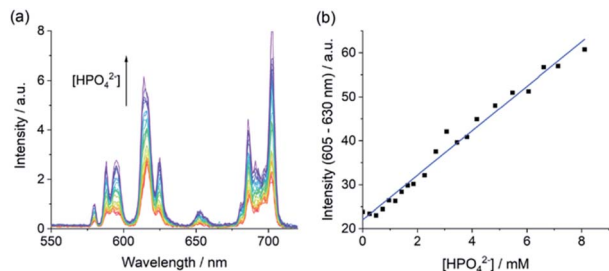
Fig. 6 Measurement of phosphate in human serum. (a) Variation in time-resolved emission spectrum of [\text{Eu}\cdot\text{Bn}]^+ (20 \mu\text{M} ) and (b) linear increase in time-resolved emission of the \Delta J = 2 band upon addition of phosphate in human serum. Measured at pH 7.0 and 295 K, \lambda_{\text{exc}} = 322 nm, integration time = 60–400 \mu\text{s} .
