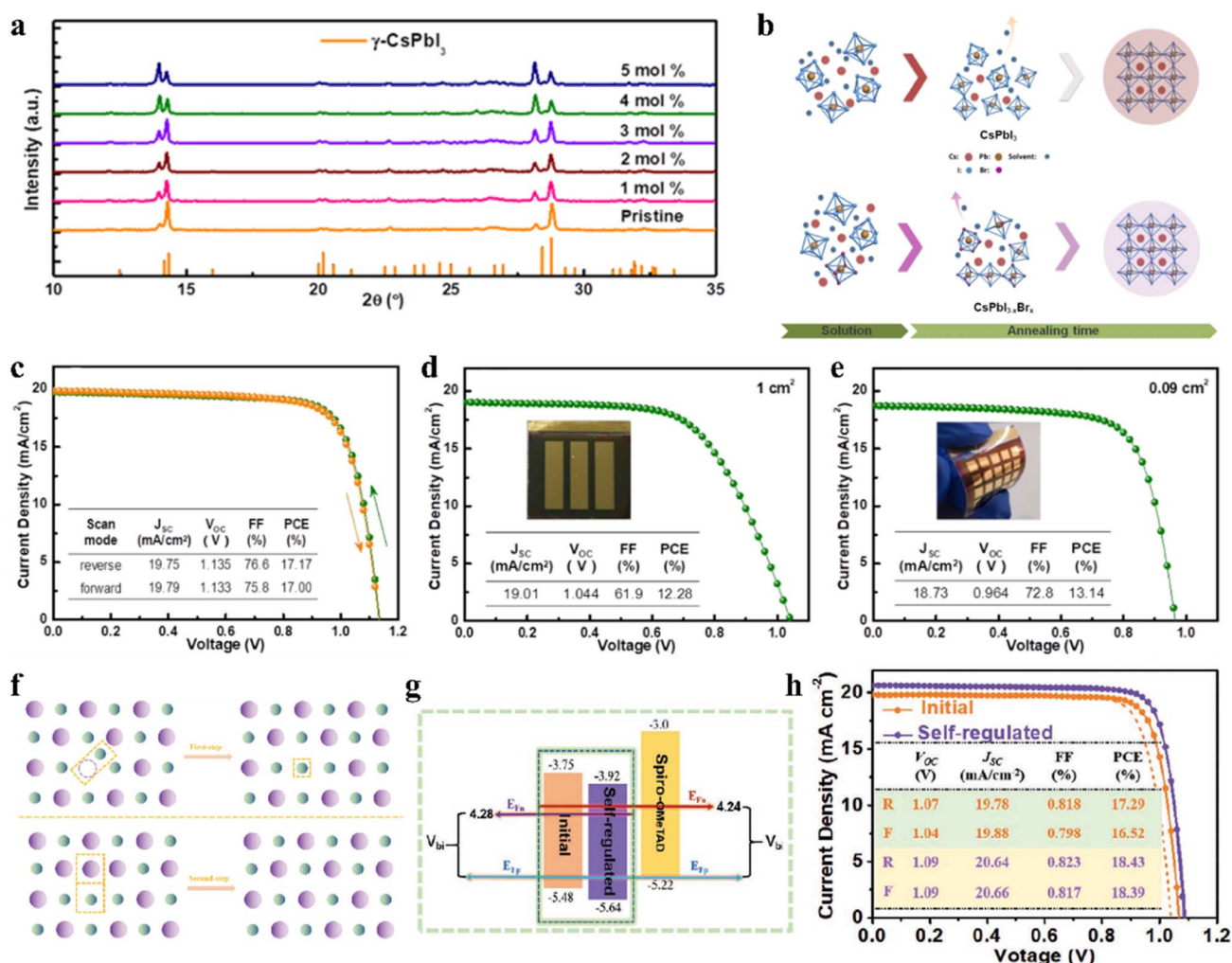
Fig. 4 (a). XRD patterns of \gamma -CsPbI 3 Cl x films. Reproduced with permission. 72 Copyright 2019, Elsevier. (b). Schematic diagram for Br-driven crystalline grain growth. J - V characteristics (c) under both the reverse and forward scan directions with an active area of 0.09 cm 2 ; (d) on a glass substrate with an area of 1 cm 2 ; and (e) on a PET/ITO/TiO 2 substrate with an area of 0.09 cm 2 . (b–e) Reprinted with permission. 76 Copyright 2019, the American Chemical Society. (f). Proposed schematic diagram of defect-regulation processes. (g). Schematic illustration of energy levels and V_{bi} . (h). J - V characteristics measured in the forward and reverse directions under AM1.5G illumination. (f–h) Reproduced with permission. 78 Copyright 2021, Wiley-VCH.
