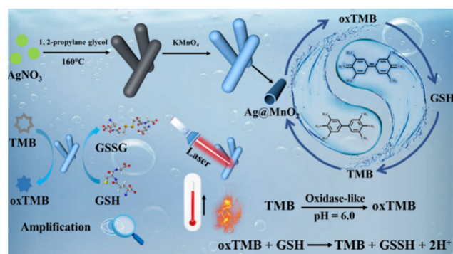
Scheme 1 Schematic illustration of the synthesis of Ag@MnO 2 nanowires and the process of dual-mode colorimetric and photothermal detection for GSH.
