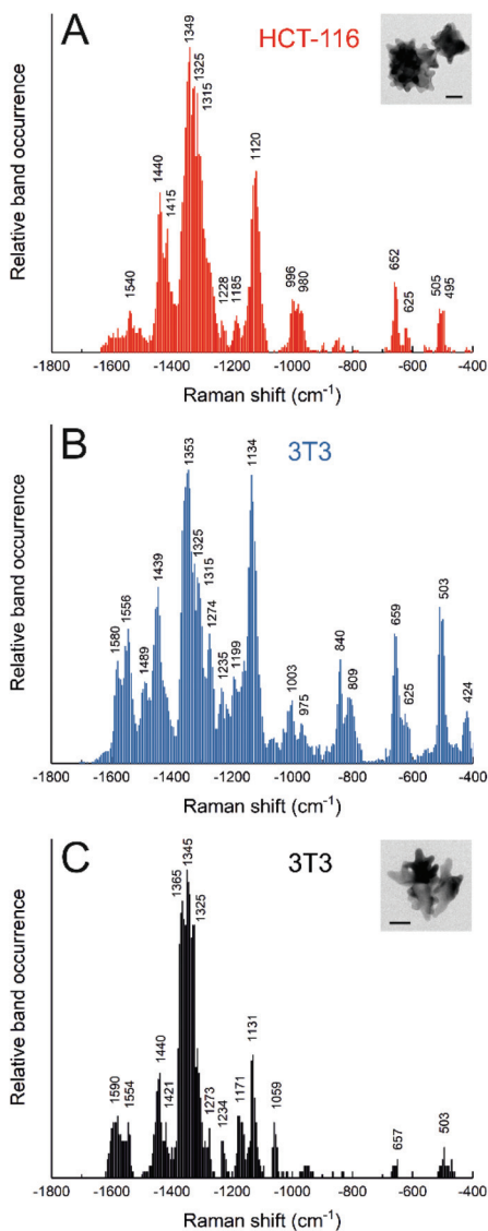
Fig. 3 Relative band occurrence in SERS spectra from (A) HCT-116 cells incubated for 24 h with gold nanostars synthesized with 25 mM HEPES; (B) 3T3 cells incubated for 24 h with gold nanostars synthesized with 25 mM HEPES; (C) 3T3 cells incubated for 24 h with gold nanostars synthesized with 75 mM HEPES. Insets: TEM micrographs of gold nanostars synthesized with 25 mM HEPES (A) and 75 mM HEPES (C) that were shown to have different tip length. Adapted from ref. 40 with permission from the Royal Society of Chemistry. Copyright 2020 RSC.
