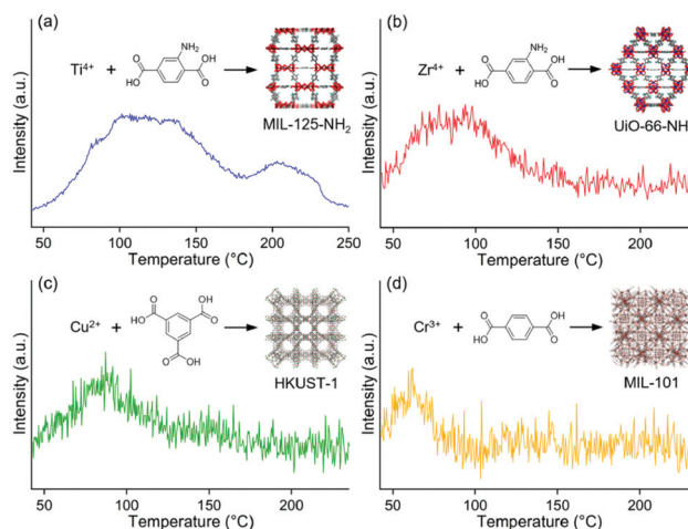
Fig. 11 TPD-MS charts of (a) MIL-125-NH 2 , (b) UiO-66-NH 2 , (c) HKUST-1, and (d) MIL-101 at m/z 60 (for AcOH molecule). This figure has been reproduced from ref. 45 with permission from the American Chemical Society, copyright 2021.
