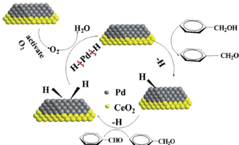
Fig. 44 Mechanism of the green oxidation method for benzyl alcohol with Pd/ \text{Fe}_3\text{O}_4 @ \text{mCeO}_2 yolk-shell microsphere catalyst. This figure was adapted with permission from Catalysis Letters , 2016, 146, 1321–1330. 283
