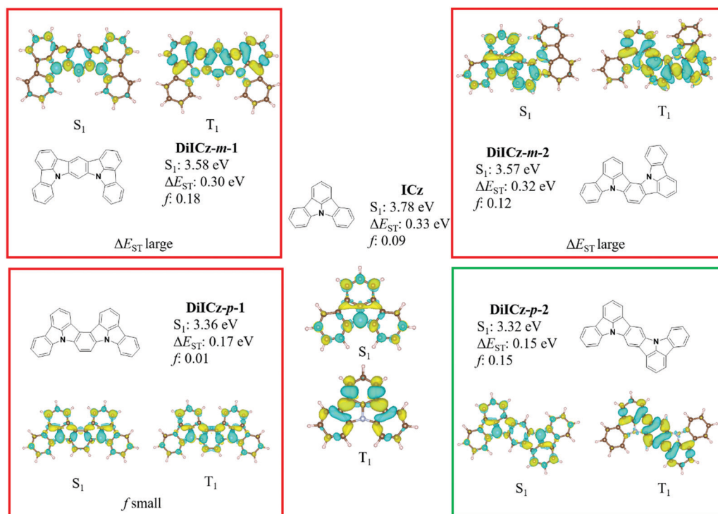
Fig. 2 S_1 and T_1 difference density patterns, \Delta E_{ST} , S_1 energy and oscillator strength, f , for the proposed DilCz units.
