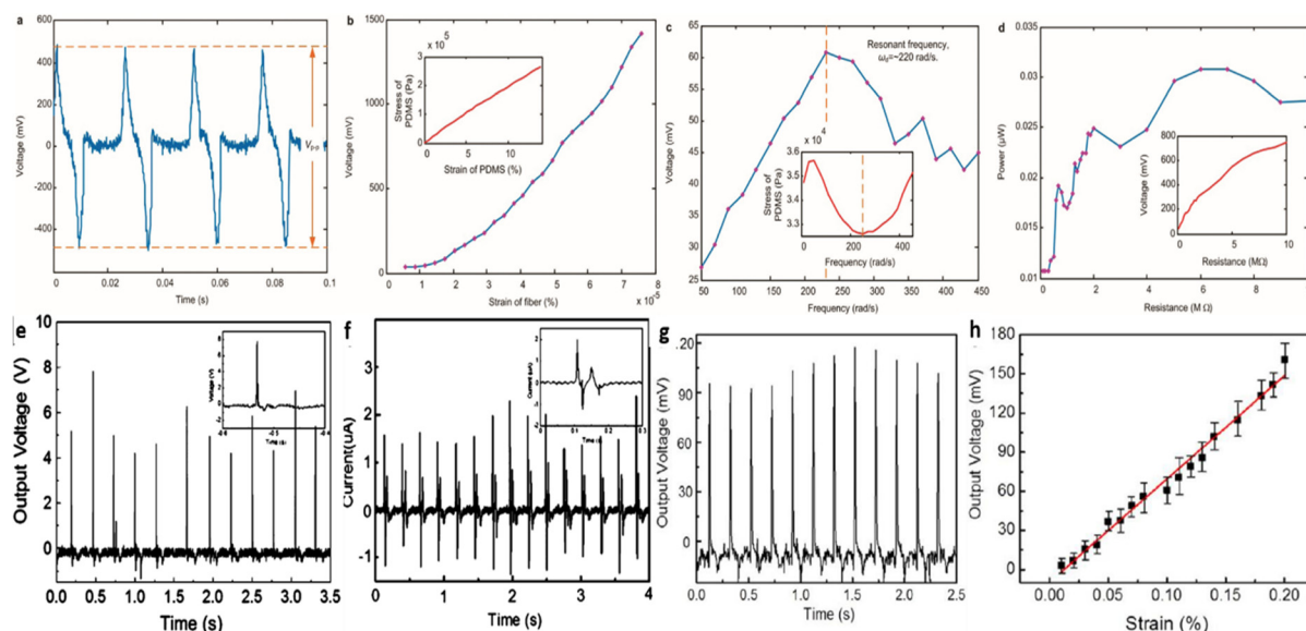
Fig. 19 (a) and (b) PZT nanogenerator output voltage with respect to time (a) and % fiber strain (b); (c) voltage with different load frequencies in the polymer matrix; (d) output power against load resistance; reproduced with permission from ref. 117. Copyright 2010, ACS Publication. Voltage (e) and current (f) generation from tapping of the PMN-PT based device with a plastic screwdriver handle; and (g) and (h) mechanical response of the PENG upon the application of cyclic stepwise strain; reprinted with permission from ref. 304. Copyright 2013, ACS Publication.
