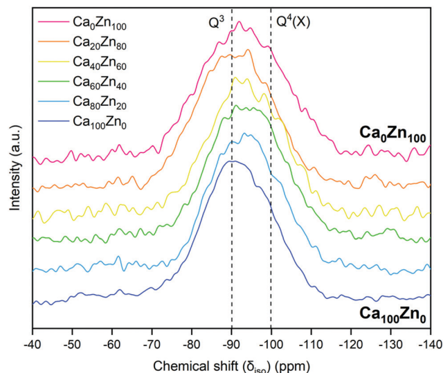
Fig. 8 ^{29}Si MAS NMR spectra for the Ca_xZn_y glass series overlaid with chemical shifts approximately representative of Q^3 and Q^4(X) (where X is a network former other than Si) species. Indicative location of Q^3 and Q^4(X) species are shown.
