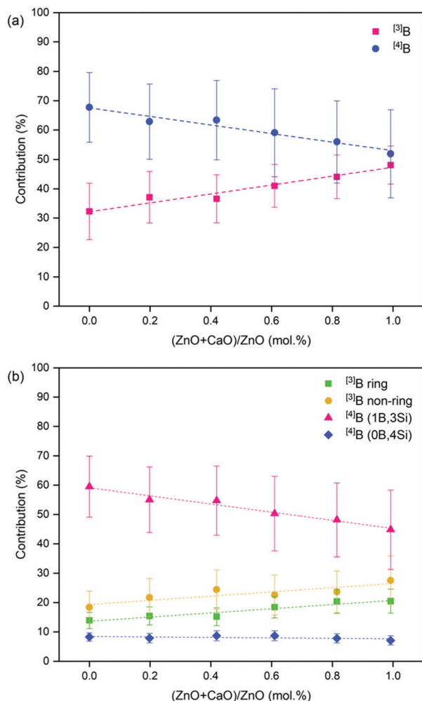
Fig. 7 Deconvolution of the ^{11}B MAS NMR spectra for the Ca_xZn_y glass series. Showing (a) total [3]B and [4]B contribution; and (b) the proportion of individual [3]B and [4]B contributions.
