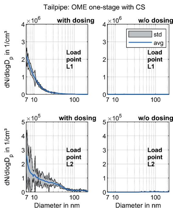
Fig. 7 Particle size distribution of OME tailpipe exhaust with and without urea dosing and one-stage dilution with volatile particle remover: filtered average (arithmic mean) of three recordings and indication of the standard deviation.
