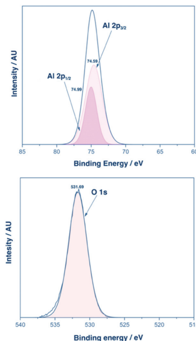
Fig. 5 XPS analysis of an \alpha\text{-Al}_2\text{O}_3 film deposited from complex 3-Al . Top: XPS of the Al 2p 1/2 and 2p 3/2 states. Bottom: XPS of the O 1s state.
