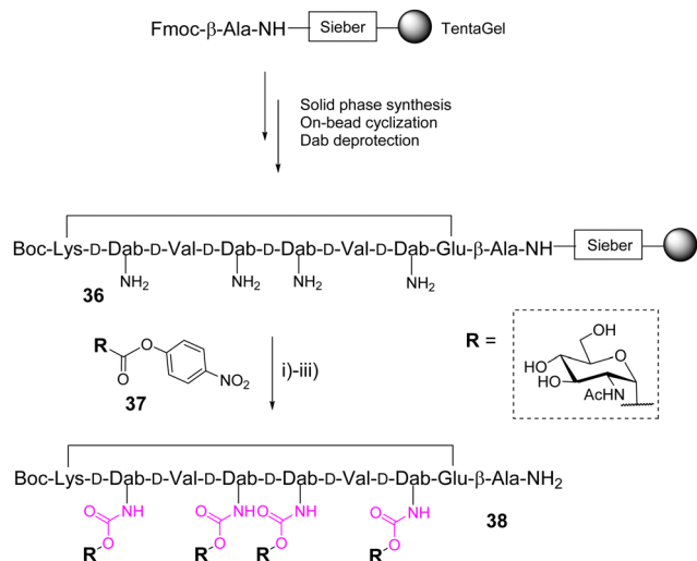
Scheme 6 On-bead synthesis of a glycosyl carbamate-cyclopeptide 38 using glycosyl p -nitrophenyl carbonate 37 . Reagent and conditions: 37 , DIPEA, NMP; (ii) \text{TFA}/\text{TIS}/\text{CH}_2\text{Cl}_2 (1 : 1 : 98); (iii) \text{NaOMe} , \text{MeOH}/\text{CHCl}_3 , 15%. Abbreviations: DIPEA: diisopropylethylamine; NMP: N -methylmorpholine.
