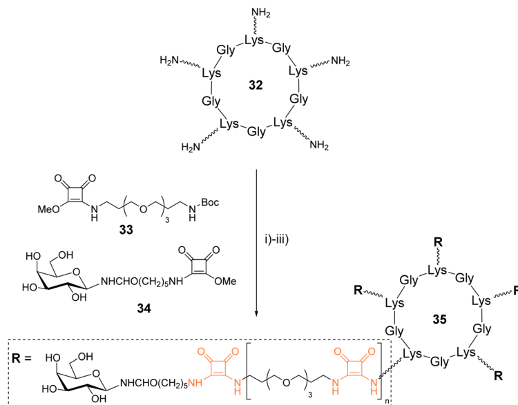
Scheme 5 Synthesis of glycoclusters using squaramide coupling. Reagents and conditions: (i) 33 , \text{NaHCO}_3 , \text{H}_2\text{O}/\text{CH}_3\text{OH} ; (ii) \text{TFA}/\text{CH}_2\text{Cl}_2 ; (iii) 34 , \text{NaHCO}_3 , \text{H}_2\text{O}/\text{CH}_3\text{OH} , approx. 70%.
