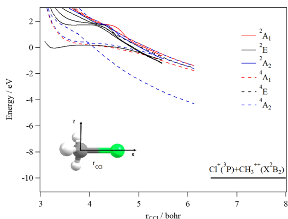
Fig. 9 spd(f) cc-pV5Z MRCI one-dimensional cuts of the PESs of the doublet and quartet states of \text{CH}_3\text{Cl}^{3+} by lengthening the r_{\text{CCl}} distance (top) and by lengthening the r_{\text{CH}} distance (bottom). The remaining coordinates were set to their equilibrium values in \text{CH}_3\text{Cl} ( X^1A_1 ). These curves are given relative to the energy of the lowest \text{CH}_3\text{Cl}^{3+} doublet state at the \text{CH}_3\text{Cl} ( X^1A_1 ) equilibrium.
