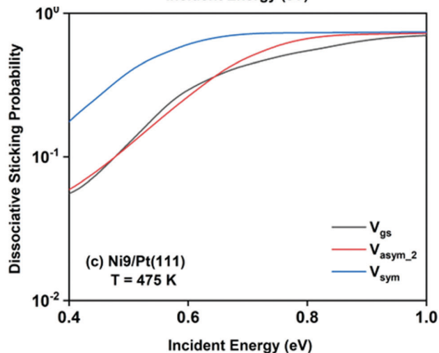
Fig. 8 Full coupling dissociative sticking probabilities, i.e. , reaction probabilities after site averaging as a function of incident energies for the ground vibrational state and one-quantum excitation in symmetric and asym 2 stretching modes of CH 4 on the three alloy surfaces at 475 K surface temperature for the dissociation of methane on (a) Sub-Pt9/Ni(111), (b) Ni8/Pt(111), and (c) Ni9/Pt(111) alloy surfaces.
