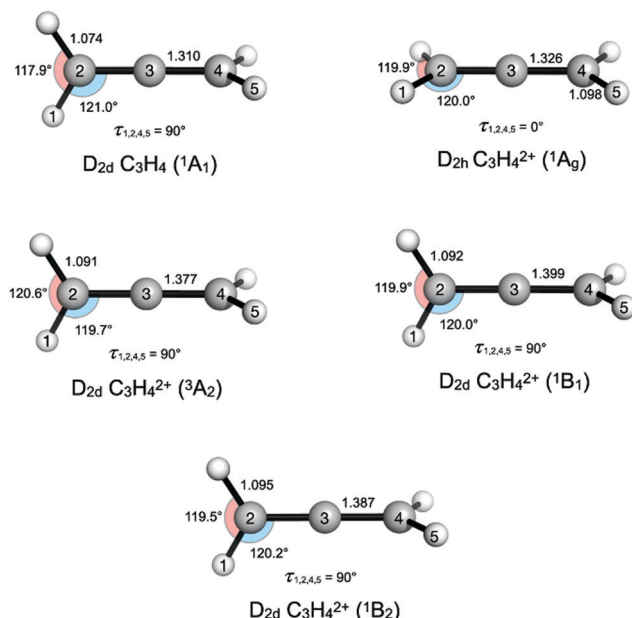
Fig. 1 Changes in electronic structure of neutral D_{2d} allene upon vertical double ionization (in eV) to the four lowest energy states to give: ^3A_2 , ^1A_1 , ^1B_1 and ^1B_2 that make up the first peak in the double ionization spectrum in Fig. 2. The D_{2d} ^1A_1 state undergoes a geometric distortion from D_{2d} \rightarrow D_{2h} to remove orbital degeneracy. Optimised geometries at the CASSCF/def2-TZVP level are shown, with distances in Å and angles in degrees.
