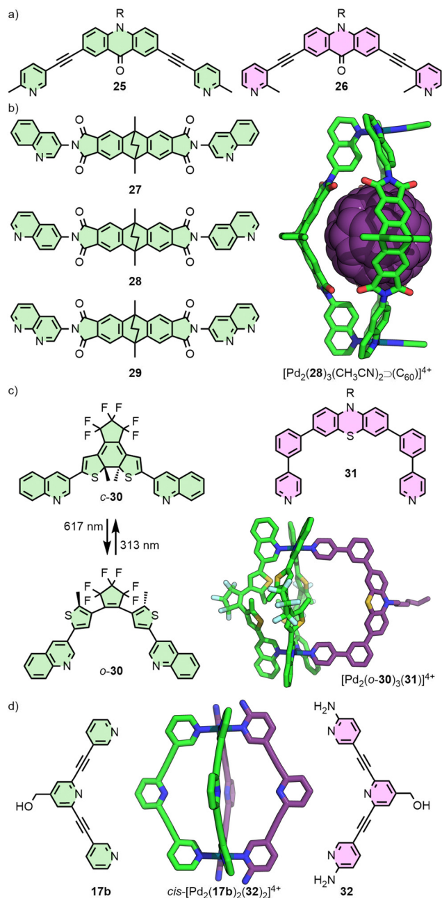
Fig. 7 Coordination sphere engineering of heteroleptic cages using the steric bulk of (a) complementary picoline-based ligands ( 25 and 26 ), and quinoline donors ( 27 , 28 and 30 ); SCXR structure of [\text{Pd}_2(\mathbf{28})_3(\text{CH}_3\text{CN})_2 \supset \text{C}_{60}]^{4+} shown in combination with ligands with (b) appropriate hydrogen-bond acceptor units ( 29 ) or (c) less sterically demanding ligands ( 31 ; SCXR structure of [\text{Pd}_2(\mathbf{o-30})_3(\mathbf{31})]^{4+} shown). (d) Heteroleptic cage \text{cis-}[\text{Pd}_2(\mathbf{17b})_2(\mathbf{32})_2]^{4+} (DFT structure with \text{CH}_2\text{OH} units omitted) was accessed through post-synthetic ligand displacement of homoleptic cage [\text{Pd}_2(\mathbf{17b})_4]^{4+} .
