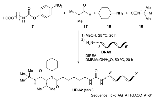
Scheme 3 Urea bond formation using DNA 3 which contains an aminohexyl linker introduced via a 3'-terminal phosphodiester bond.
